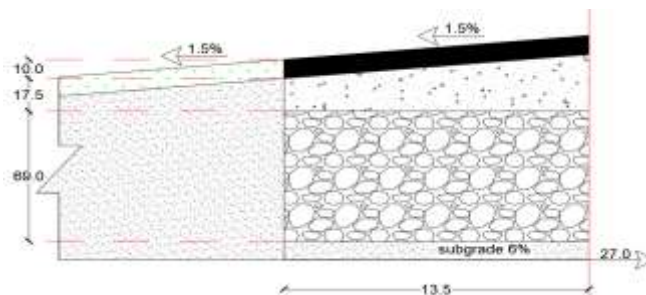
Gambar 4. Desain slope taxiway
